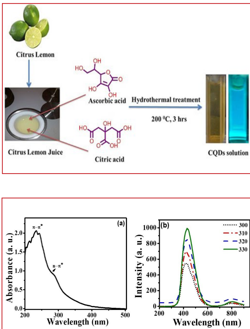
Figure 4. (a) UV-Vis spectrophotometric absorption spectrum of CQDs. (b) Photoluminescence spectrum (PL) of CQDs With different excitation beams
