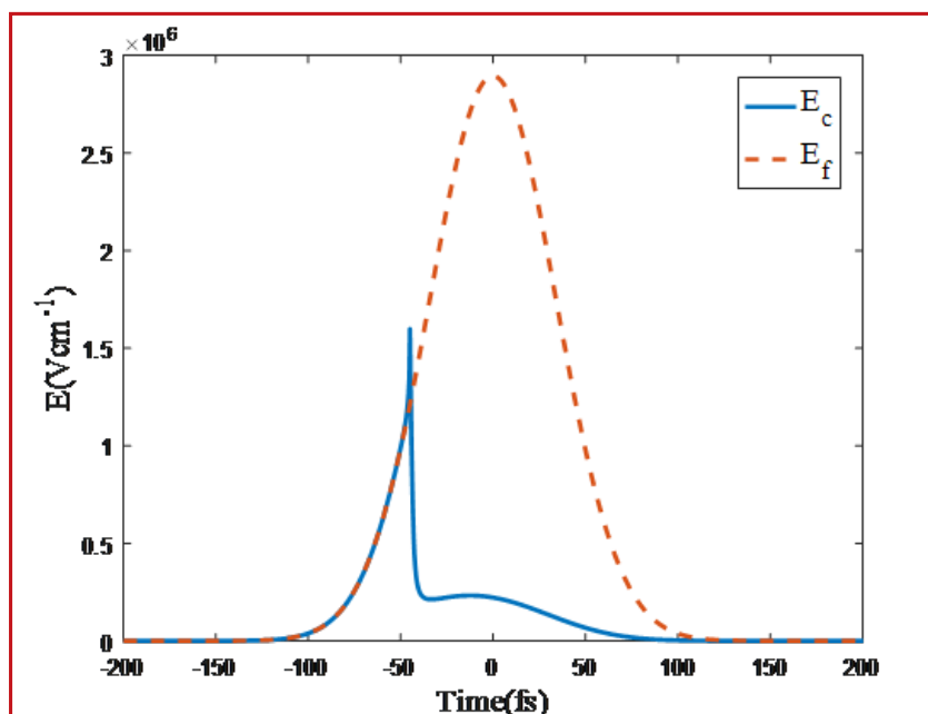
Chart 2. The laser's electric field with 40fs pulse duration, 825 nm wavelength, and with intensity 1 \times 10^{15} \text{ W cm}^{-2} (dashed) and electric field inside the cluster in laser interaction (solid)
